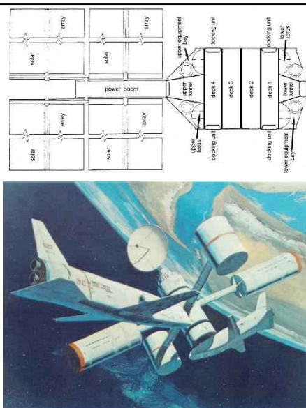
Figure 27: North American Rockwell's 12-man design (top) and 100-man design (bottom).
