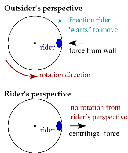
Figure 16: The difference between centripetal (actual) and centrifugal (apparent) acceleration.
