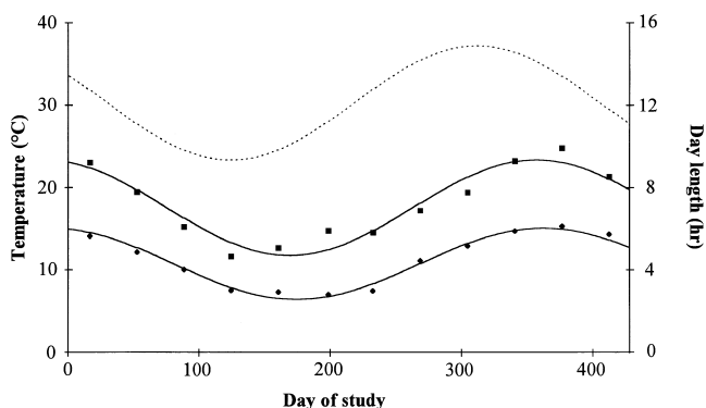
FIG. 1. Day length at long. 175^{\circ}38'E , lat. 40^{\circ}22'S (---), average minimum (◆) and maximum (■) monthly temperatures and the sine-functions fitted to the day length (---) and minimum and maximum daily temperature (—) data.
