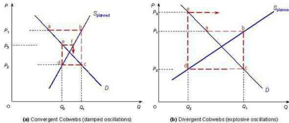
Figure 2.3 Illustration of Cobweb Model
