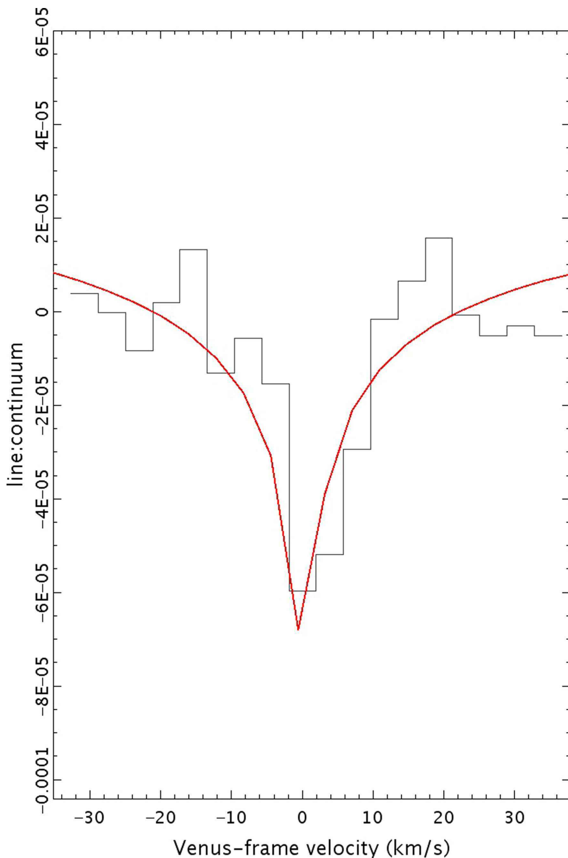
Extended Data Fig. 5 | Deuterated water (HDO) is detected on Venus in the ALMA data. A preliminary reduction of the whole-planet spectrum in the HDO 2_{2,0}-3_{1,3} transition is shown. The overlaid red curve is from our radiative transfer model, calculated for 2.5 ppb abundance and processed with a 1 st -order polynomial fit, as for the data. No correction has been made for line-dilution, so the abundance can be significantly under-estimated, depending on the scale over which the molecules are distributed.
