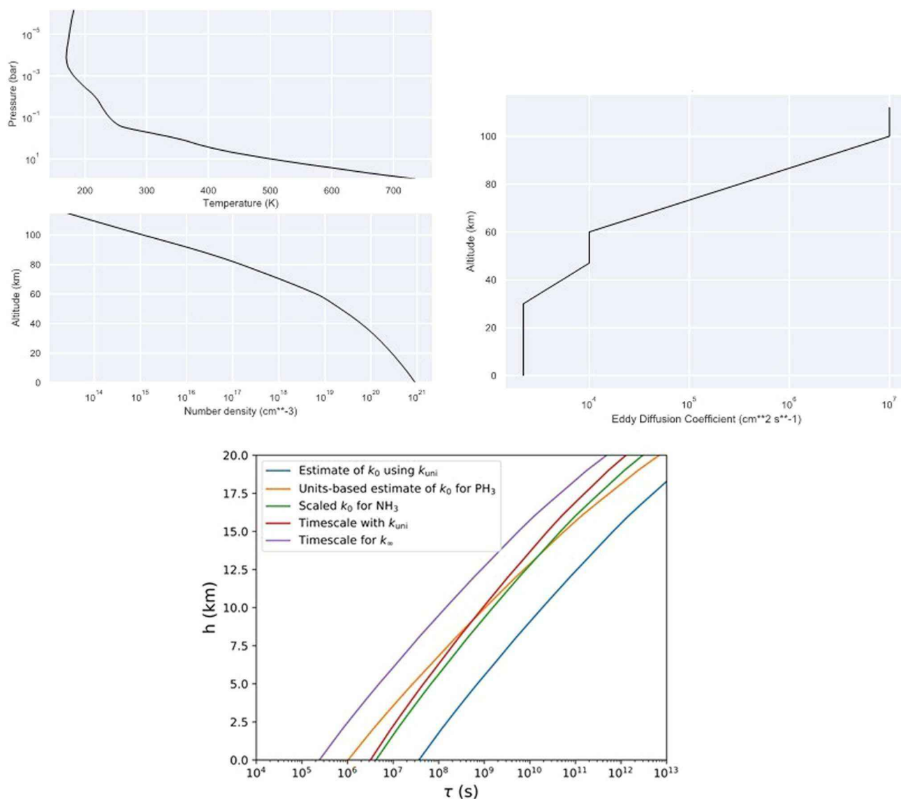
Extended Data Fig. 8 | Inputs to the photochemical modelling are illustrated. Top-left panel: Temperature-pressure profile used in photochemical modelling of the Venusian atmosphere, following refs. 46,56 . Top-right panel: Eddy diffusion profile used here in photochemical modelling of the Venusian atmosphere, following refs. 46,56 . Lower panel: Decomposition timescale for \text{PH}_3 as a function of height, derived from the Lindemann approximation of the rate constant, employing a theoretical value of k_{\infty} ( \text{s}^{-1} ) and an approximation of k_0 ( \text{cm}^3 \text{s}^{-1} ) using k_{\text{uni}} ( \text{s}^{-1} , blue), a simple unit-conversion estimate of k_0 (orange), a scaled estimate of k_0 based on ammonia decomposition (green), the timescale using only k_{\text{uni}} (red), and the timescale at the high pressure limit (violet).
