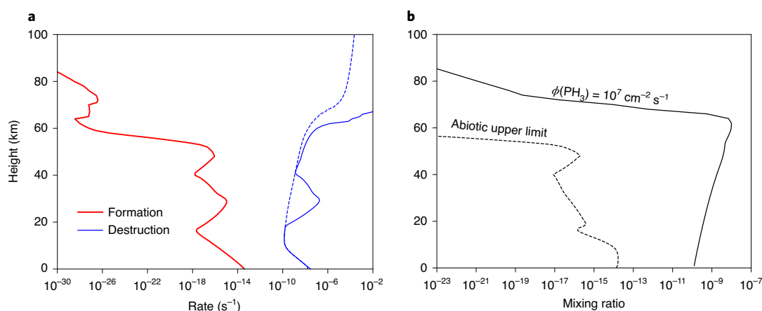
Fig. 5 | Predicted maximum photochemical production of \text{PH}_3 found to be insufficient to explain observations by more than four orders of magnitude. a , Upper limits of the predicted photochemical production rates of \text{PH}_3 (excluding transport; red curve, \text{s}^{-1} ) compared with photochemical destruction rates (blue curve, \text{s}^{-1} ), including radicals and atoms (blue solid) and ignoring radicals and atoms (blue dashed), as a function of height (km). See kinetic network of Extended Data Fig. 7. b , Mixing ratio of \text{PH}_3 as a function of atmospheric height (km), for a production flux ( \phi(\text{PH}_3) ) within the cloud layer (~55–65 km) of 10^7 \text{ cm}^{-2} \text{ s}^{-1} (solid curve), compared with the predicted steady-state abiotic upper limit (dashed curve). See kinetic network of Extended Data Fig. 7.
