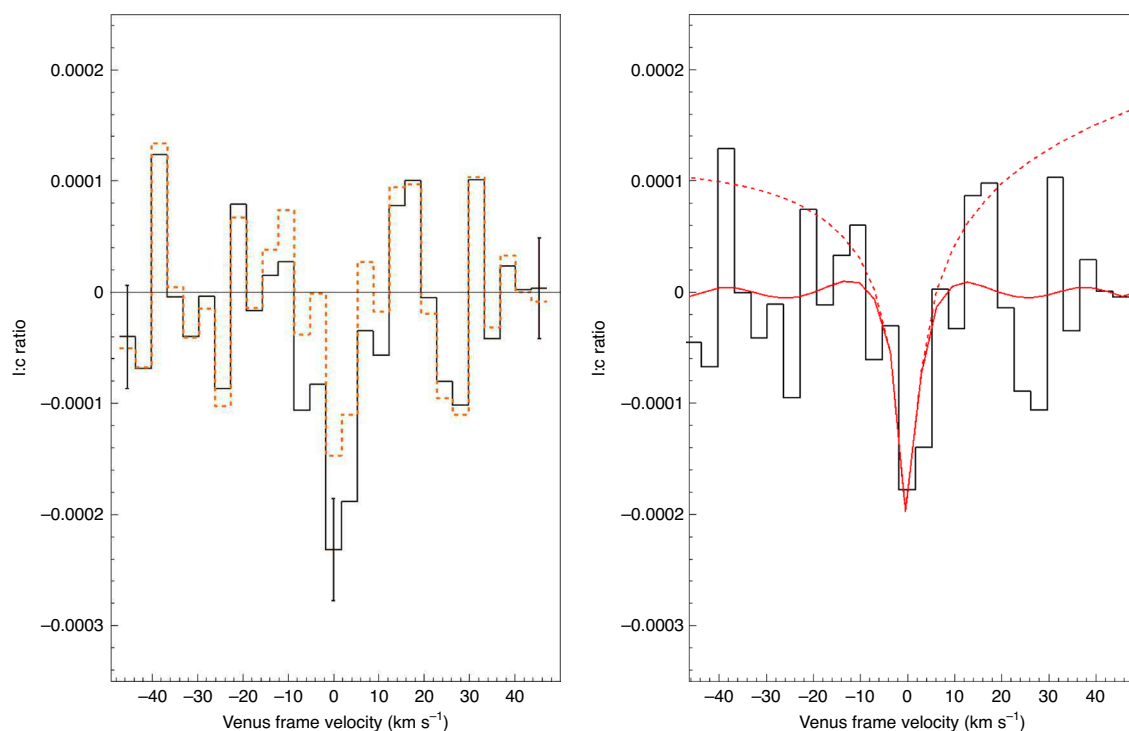
Fig. 1 | Spectra of \text{PH}_3 1–0 in Venus’s atmosphere as observed with the JCMT. Axes are l:c ratio against Doppler-shifted velocity referenced to the \text{PH}_3 wavelength. Left: the least and most conservative solutions after fitting and removing spectral ripple (see ‘JCMT data reduction’ in Methods), with the residual line present inside velocity ranges of |v| = 8 \text{ km s}^{-1} (solid, black) and |v| = 2 \text{ km s}^{-1} (dashed, orange). The data have been binned for clarity into histograms (that is, bars denoting averages) on the x axis; representative 1\sigma error bars are 0.46 \times 10^{-4} in l:c ratio per 3.5 \text{ km s}^{-1} spectral bin. Error bars indicate the dispersion within each channel from 140 co-added input spectra; channel-to-channel dispersion is higher by \sim 40\% , attributable to residual ripple, and contributing to the range of signal-to-noise ratio (Table 1). Right: the adopted mid-range solution with |v| = 5 \text{ km s}^{-1} (histogram), overlaid with our model for 20 ppb abundance by volume. The solid red curve shows this model after processing with the same spectral fitting as used for the data. The line wings and continuum slope have thus been removed from the original model (bottom dashed red curve). As the spectral fitting forces the line wings towards zero, only the range \pm 10 \text{ km s}^{-1} around Venus’s velocity was used in line characterization (Table 1).
